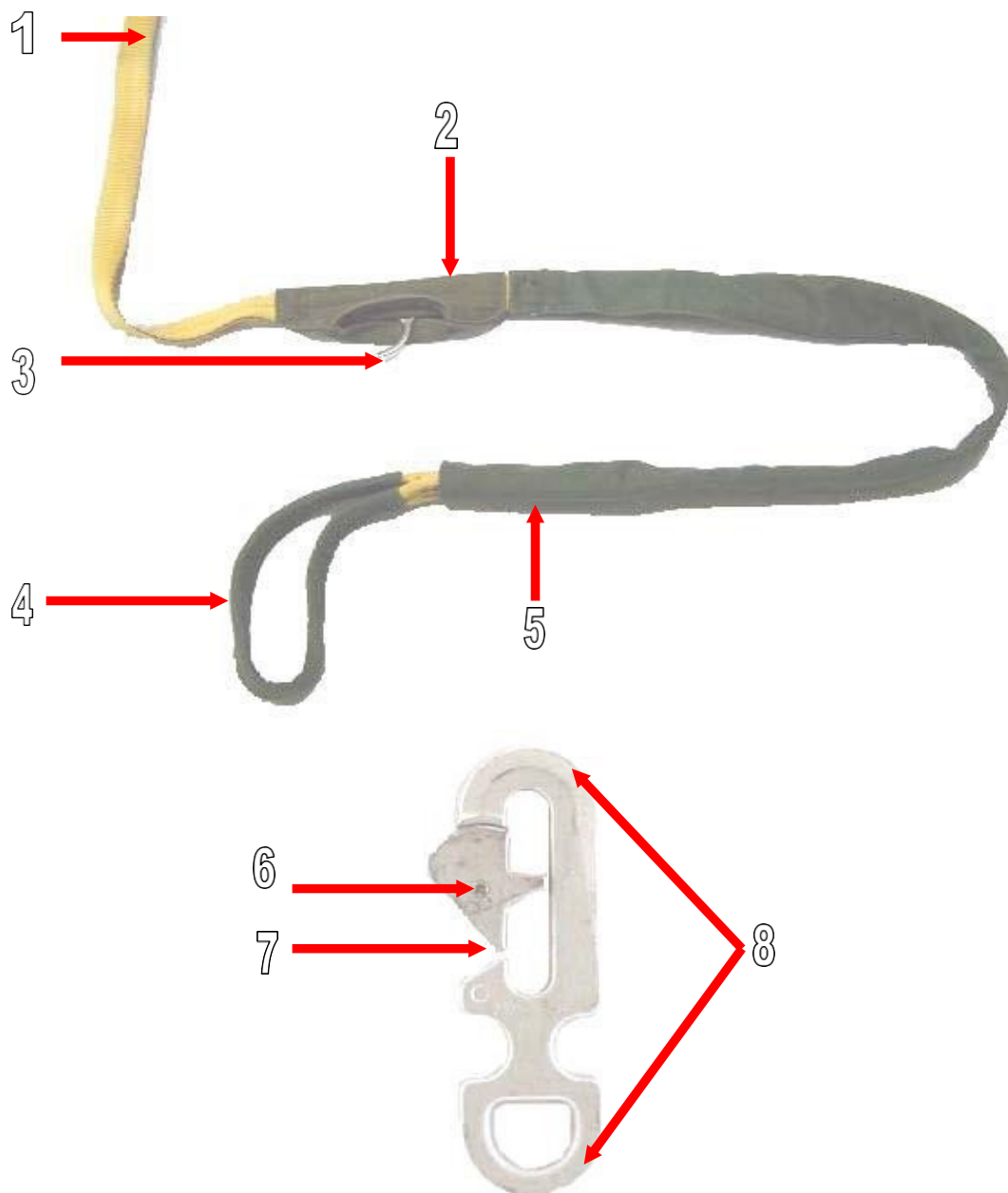
Canopy Release Assembly
