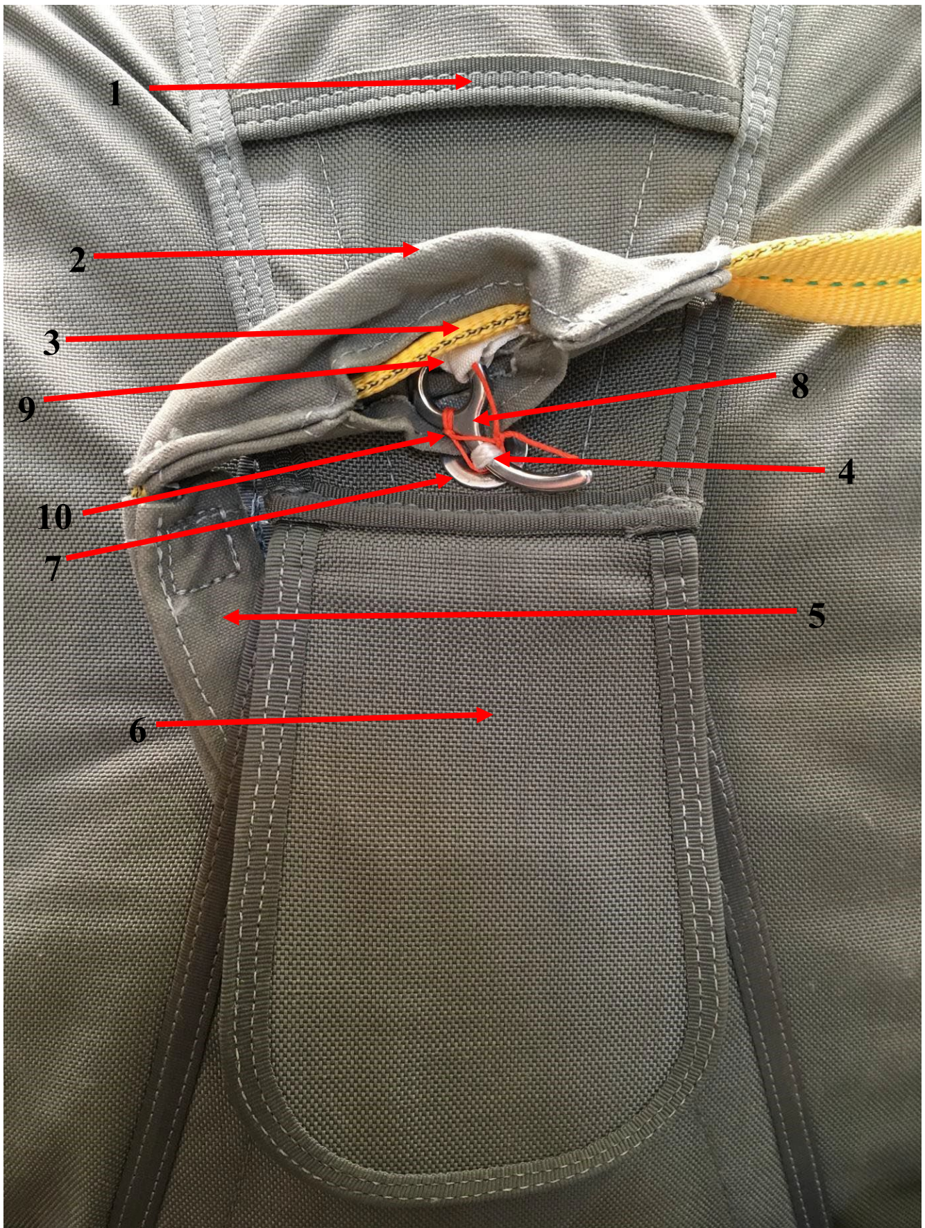
Pack Tray
